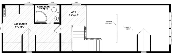
Laramie 1550-A2 2nd Floor
