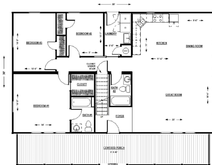
Cherokee 3050-A1 Price $269,950*
